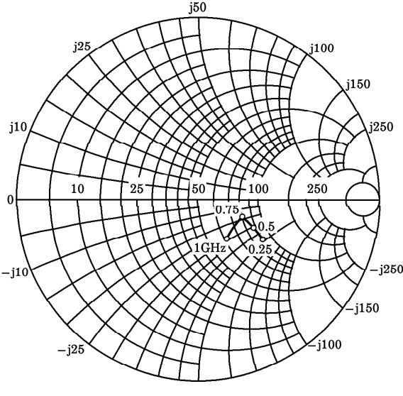
S_{22e} (UNIT : \Omega )
